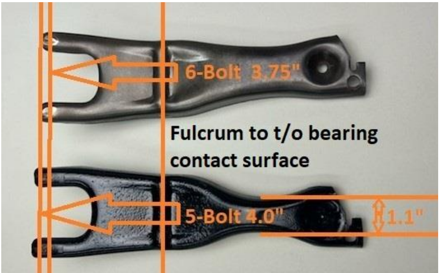
5-bolt (bottom) & 6-Bolt (top) forks shown with dimensions.
