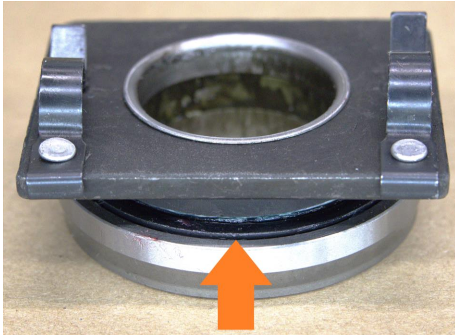
Seal Shown on the back side of the bearing, indicating constant-contact style bearing.
